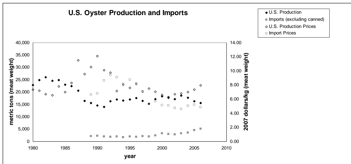
Figure 6.1. U.S. oyster production, including wild harvest and mariculture, (1980–2006) and imports (1989–2006) and prices in constant 2007 dollars. Source: National Oceanic and Atmospheric Administration (2007; 2009b, d).
