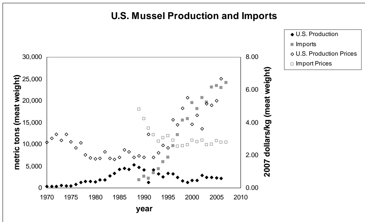
Figure 6.3. U.S. mussel production, including wild harvest and mariculture, (1970–2006) and imports (1989–2007) and prices in constant 2007 dollars. Source: National Oceanic and Atmospheric Administration (2007, 2009b, d).
