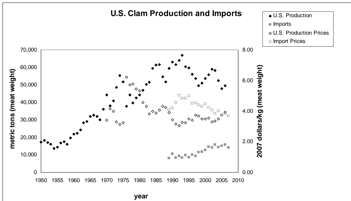
Figure 6.2. U.S. clam production, including wild harvest and mariculture, (1950–2006) and imports (1989–2007) and prices in constant 2007 dollars. Production data include quahogs, surf clams, Manila clams, soft shell clams, and geoducks. Source: National Oceanic and Atmospheric Administration (2007; 2009b, d).
