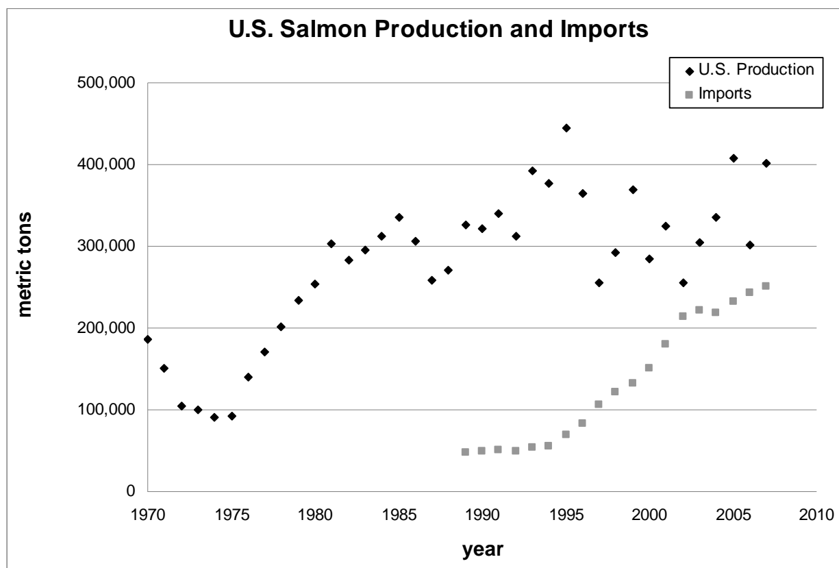
Figure 4.2. U.S. salmon landings (1970–2007) and imports (1989–2007). Source: National Oceanic and Atmospheric Administration (2007, 2009b).
