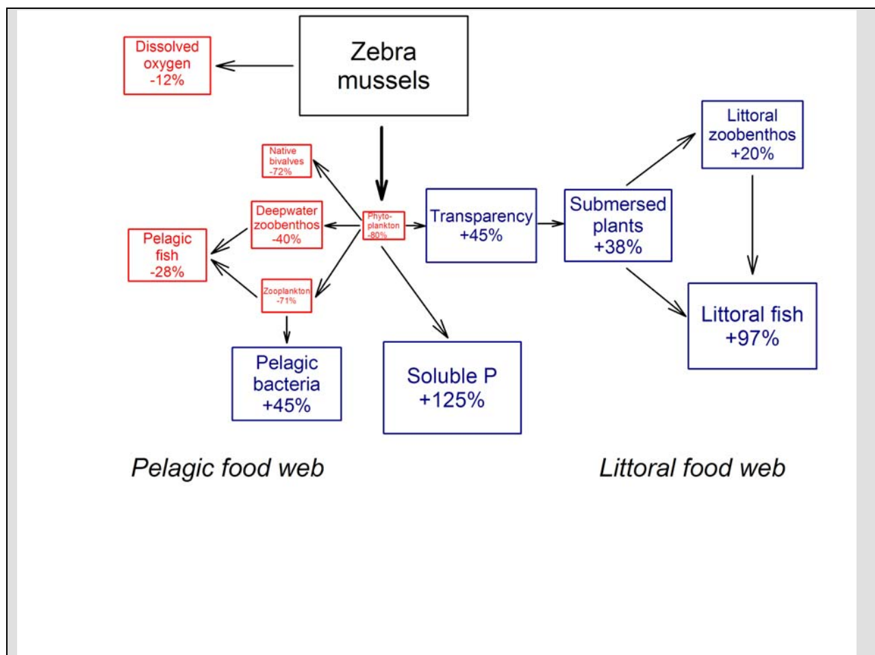
Figure 1.1. Summary of the effects of the zebra mussel invasion on the Hudson River ecosystem. The area of each box is proportional to the change in each component that was associated with the zebra mussel invasion; blue boxes show increases, whereas red boxes indicate decreases (copyright by the Ecological Society of America; Strayer, 2009).
